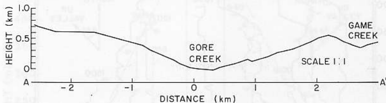
Fig. 2. Topographic cross-section AA' through the balloon profiler site normal to the valley axis
