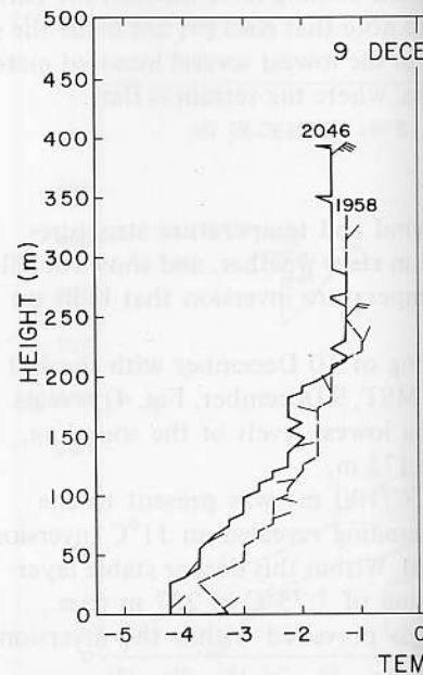
Fig. 4. Same as Fig. 3
