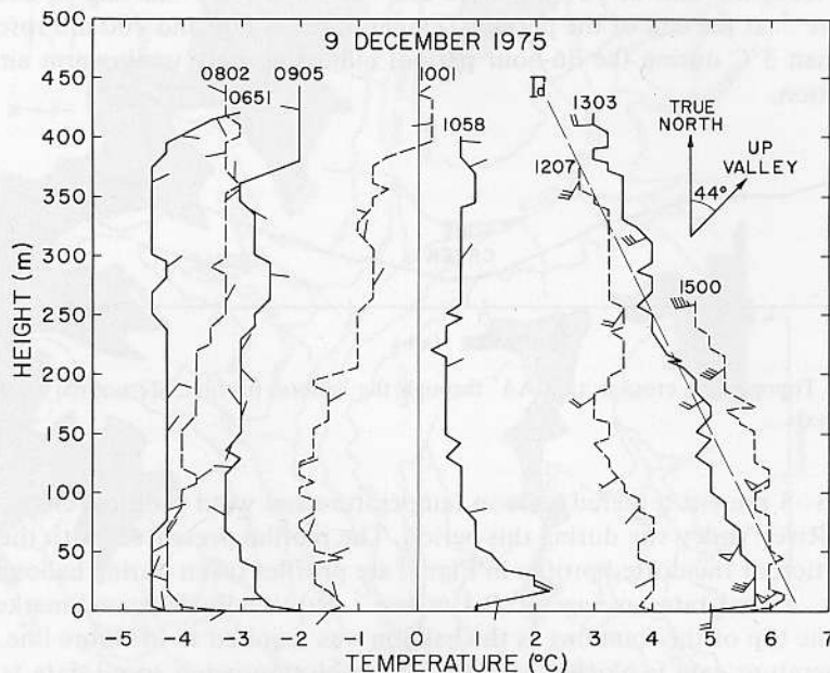
Fig. 3. Tethered balloon soundings, 9 December, 1975. Temperature soundings are shown for the times (MST) indicated. Wind directions and speeds are superimposed on the temperature soundings. A single barb indicates 1 \text{ m sec}^{-1} . Triangle indicates 5 \text{ m sec}^{-1} . The dry adiabatic lapse rate ( \Gamma_d ) is given for reference
