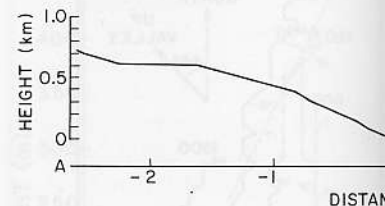
Fig. 2. Topographic cross-section AA' of the Gore River Valley axis
