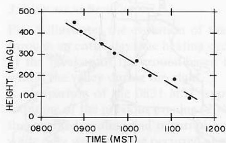
Fig. 6. Inversion top height versus time, 10 December 1975
