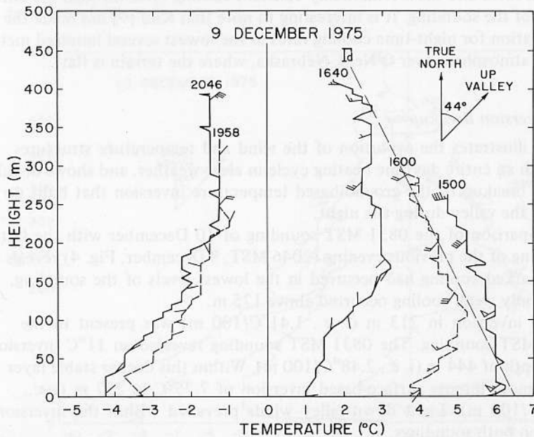
Fig. 4. Same as Fig. 3
